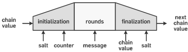
Fig. 3. BLAKE compression function
