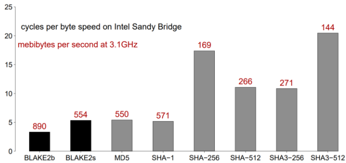
Fig. 8. Speed comparison of various popular hash functions [15]
