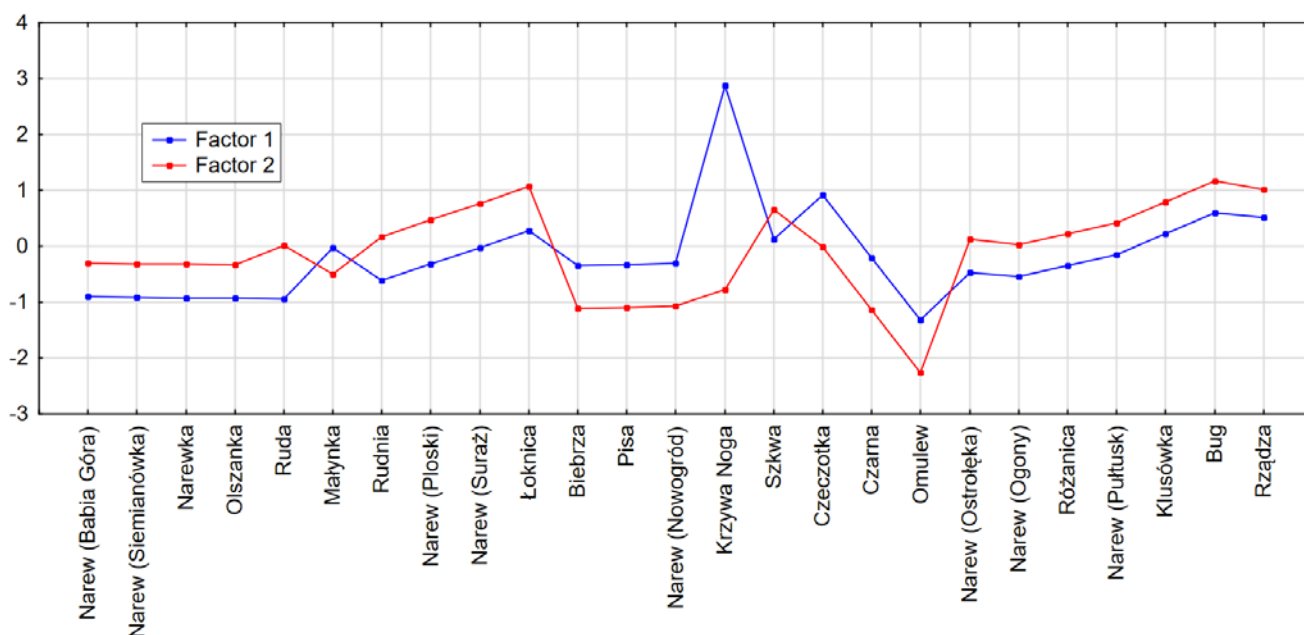
Fig. 3. Distribution of factor loads in the Narew River catchment area.
