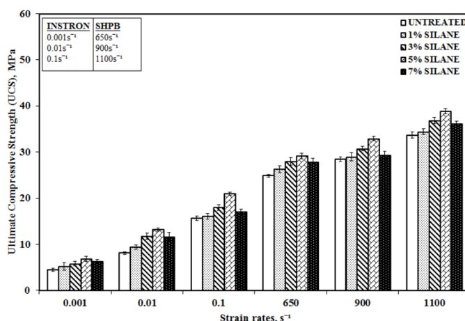
Fig. 5. The ultimate compressive strength (UCS) of the untreated LLDPE/RH and the treated LLDPE/RH composites under various loading rates
