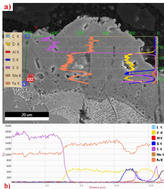
Fig. 5. Transition layer at mould/casting interface of the specimen taken from casting no. 2; a) Morphology of microstructure constituents, SEM, b) Profile of concentration of the selected elements, EDS
