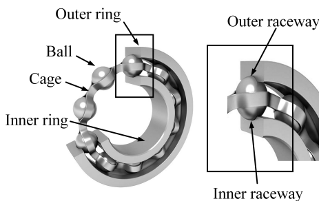
Fig. 1. Diagram of the construction of a rolling bearing [11].
