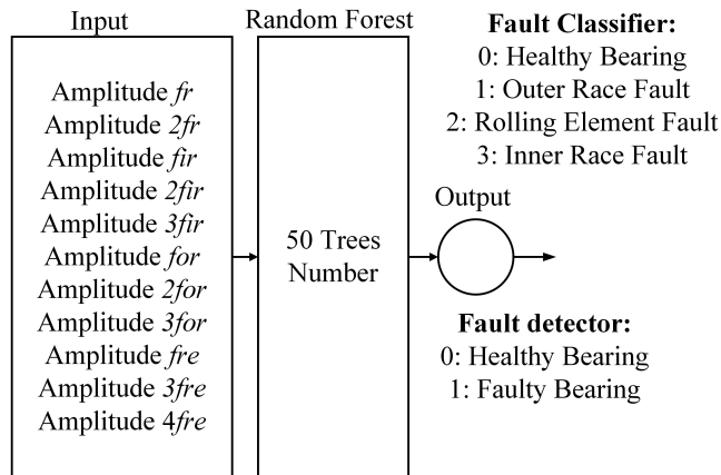
Fig. 6. Schematic diagram of RF.
