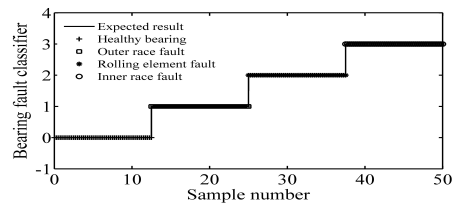
Fig. 8. Waveforms of output values of RF based on ENV.
