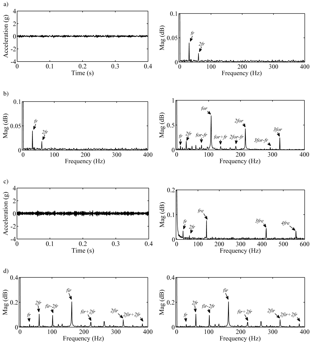
Fig. 4. Vibratory signatures and spectral envelope analysis: a) healthy bearing; b) bearing with an outer race fault; c) bearing with a rolling element fault; d) bearing with an inner race fault.
