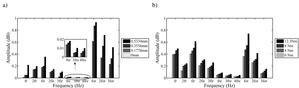
Fig. 5. Selected harmonic amplitudes of characteristic frequencies obtained using ENV for (a) different fault diameters with no-load; (b) different load torques under 0.5334 mm fault diameter.
