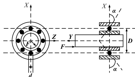
Fig. 2. Geometric characteristic of a bearing.
