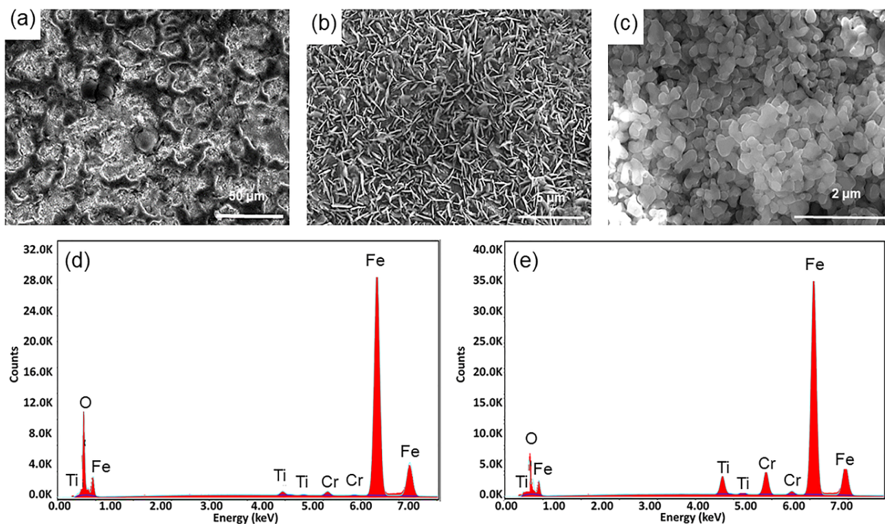
Fig. 9. SEM micrographs and EDS analysis of 24 h aged Fe-4Cr-6Ti sample isothermally oxidized at 500°C, (a) morphology of the surface, (b) adherent oxide scale (dark regions), (c) spallation region (light zones), (d) composition of the oxide scale and (e) composition of the spalled regions
