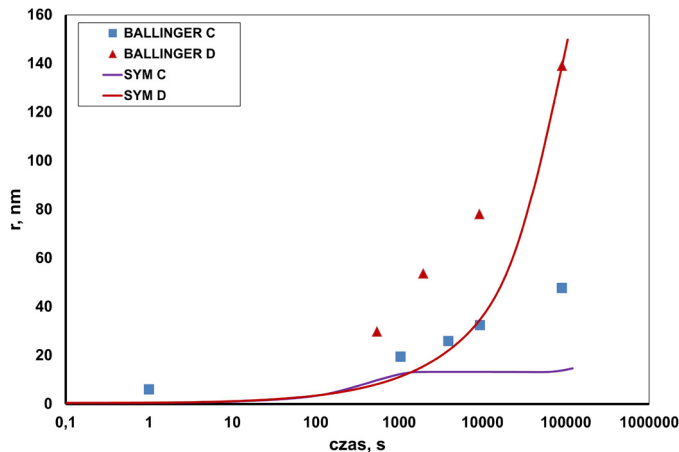
Fig. 6. Comparison of calculated mean radius, \bar{r} , (steel C – 0.02C/0.022N/0.26V and D – 0.05C/0.0002N/0.27V) of precipitation with experimental data [17], at T = 790^\circ\text{C} for t = 90000 s.
