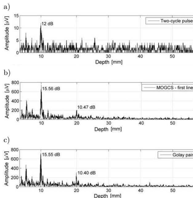
Fig. 7. Comparison of the SNR for tissue-mimicking phantom echoes obtained using the short pulse (a); the MOGCS (b); the conventional CGCS (c) transmission. The absolute values of the received echoes are shown.
