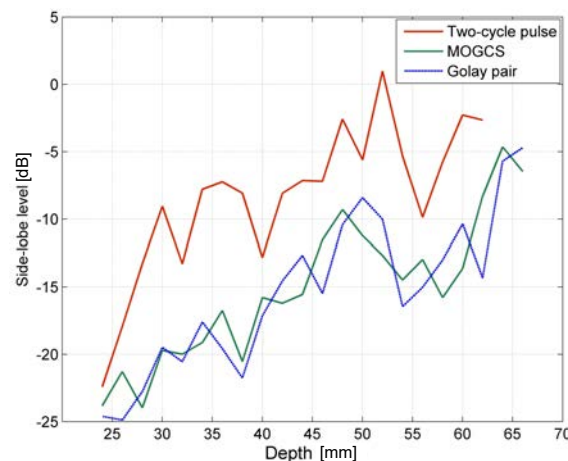
Fig. 6. The SLL vs. depth for the processed signals obtained from the wire phantom (see Fig. 5).
