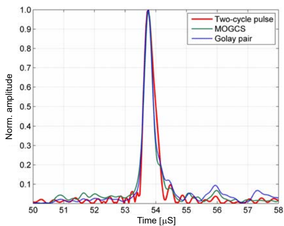
Fig. 4. Comparison of the processed RF echoes obtained from the perfect reflector using the short pulse, the MOGCS, and the CGCS transmitted signals.
