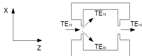
Fig.3. Dual-mode cavity
