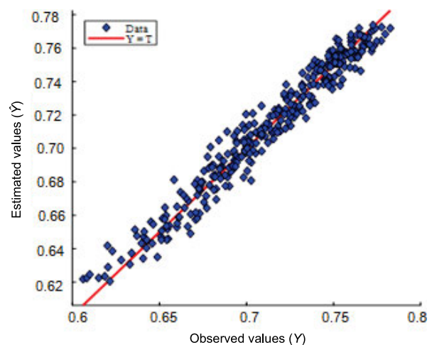
Fig. 5. Relationship between the estimated values (Ŷ) and the observed values (Y) using a neural configuration model [5-11-1] in the Rabat-Kénitra region; source: own study
