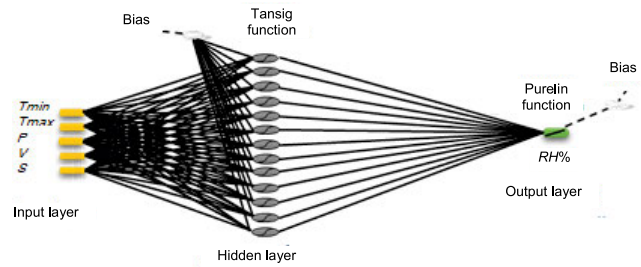
Fig. 4. Architecture of the neural network with three configuration layers [5-11-1] developed for the prediction of relative humidity (RH) in the region of Rabat-Kenitra; source: own study
