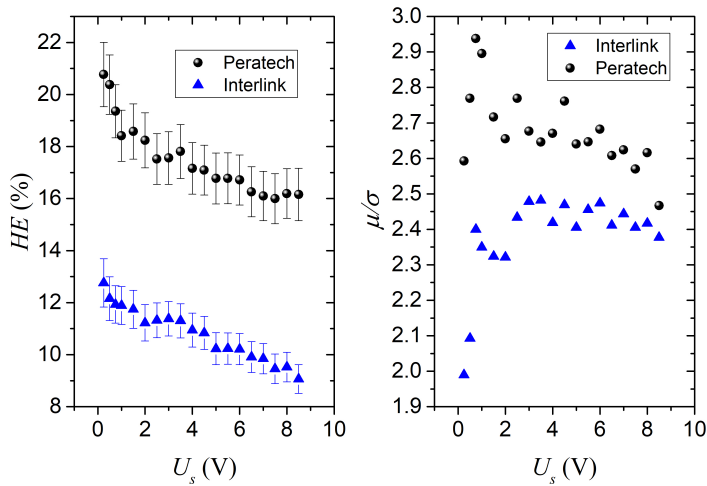
Fig. 6. Hysteresis error ( HE ) as a function of input voltage ( U_s ). Left: error bar plot comparing the HE of both sensor models. Right: dispersion in the HE calculated from the \mu/\sigma quotient.
