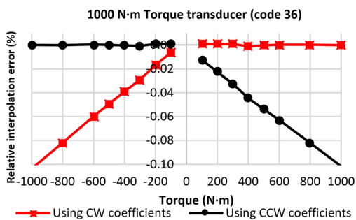
Fig. 6. Cubic relative interpolation error for the 1000 N·m torque transducer (Code 36).
