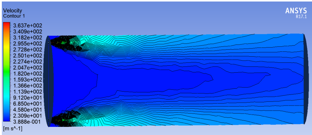
Fig. 11. Speed fields in the intersecting plane through the axis of the mixer at an angle of inclination of the nozzles of 0^\circ
