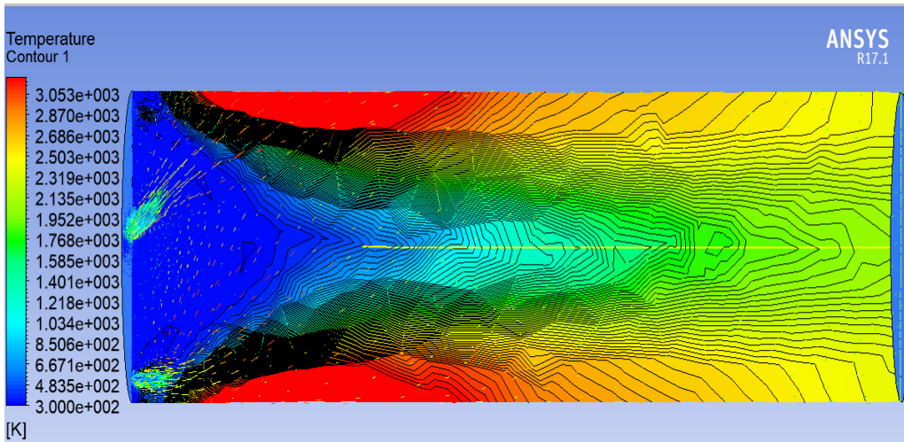
Fig. 5. Temperature fields in the intersecting plane through the axis of the mixer at an angle of inclination of the nozzles of 45^\circ
