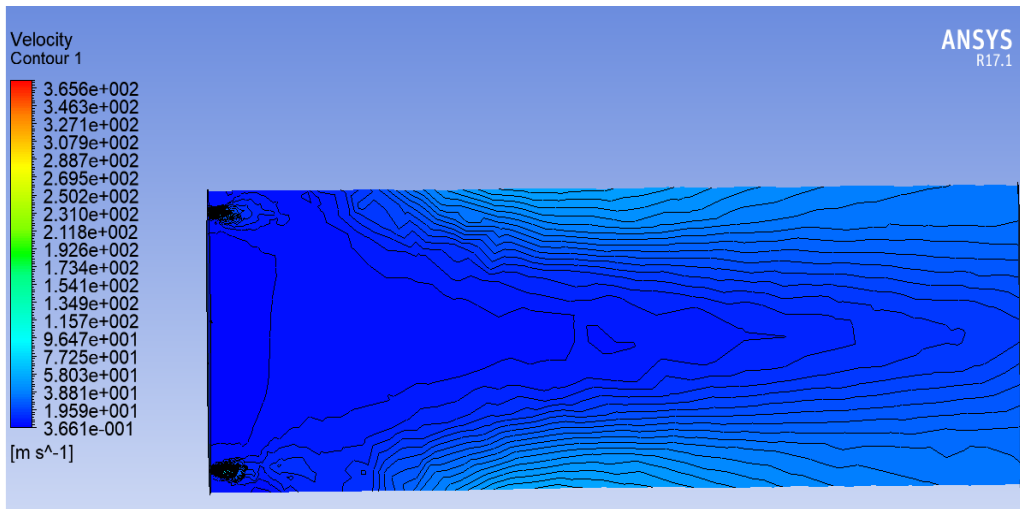
Fig. 6. Speed fields in the intersecting plane through the axis of the mixer at an angle of inclination of the nozzles of 45^\circ
