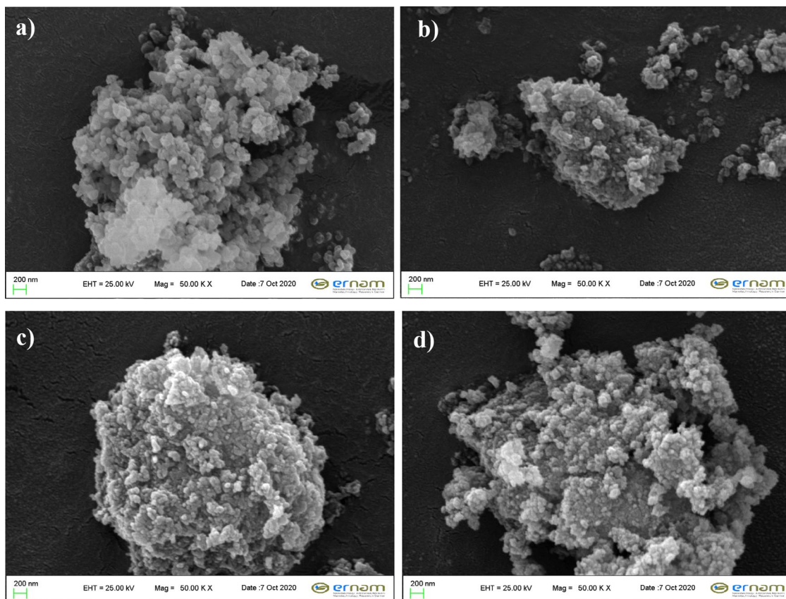
Fig. 1. SEM images of hydrothermally produced and non-heat treated Hydroxyapatite samples, 50000 \times a) 180 ^{\circ} C, 6 hour (HA-6h), b) 180 ^{\circ} C, 12 hour (HA-12h) c) 180 ^{\circ} C, 18 hour (HA-18h) d) 180 ^{\circ} C, 24hour (HA-24h)
