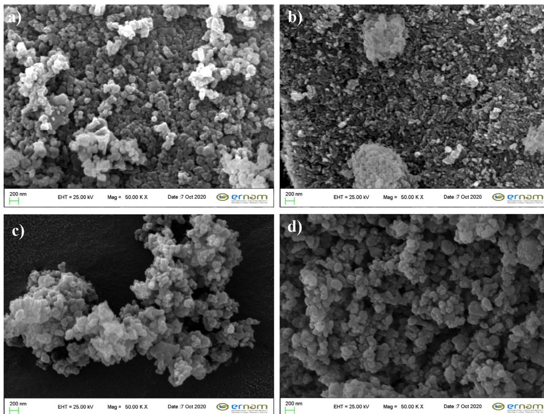
Fig. 2. SEM images of hydrothermally produced and heat treated Hydroxyapatite samples, 50000× a) 180°C, 6 hour (HA-6h-HT), b) 180°C, 12 hour (HA-12h-HT) c) 180°C, 18 hour (HA-18h-HT) d) 180°C, 24 hour (HA-24h-HT)
