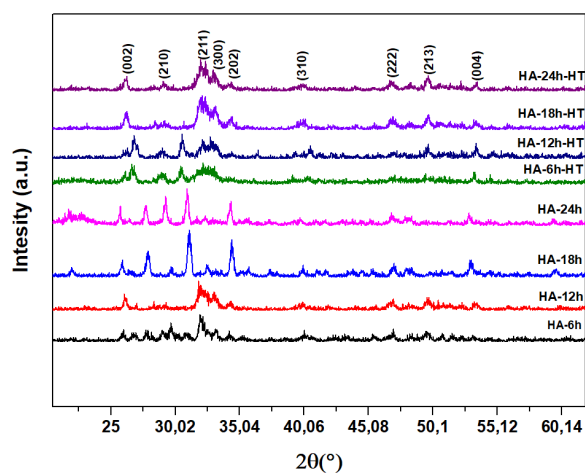
Fig. 4. X-Ray diffraction patterns of Hydroxyapatite samples
