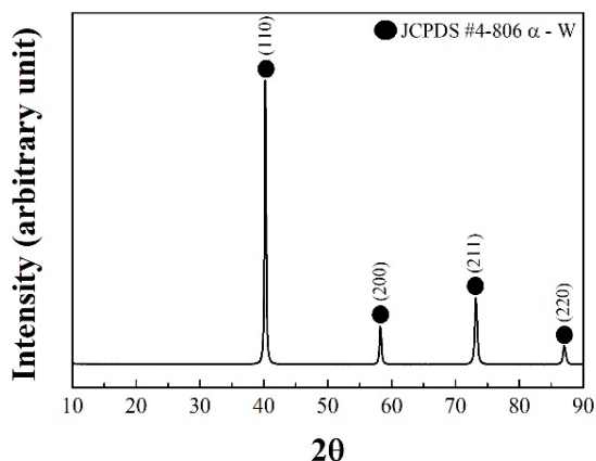
Fig. 2. XRD profile of W-1 wt% La 2 O 3 -1 wt% Y 2 O 3 powder prepared by polymeric additive solution route and hydrogen reduction
