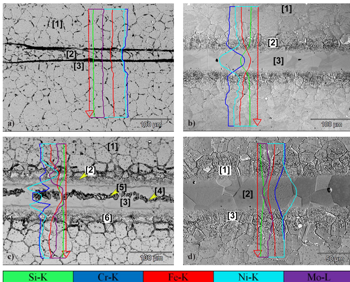
Fig. 9. Microstructure (SEM) and linear elements distribution for Hastelloy X/Amdry 915 joints for brazing processes interrupted at: a) 1050°C, c) 1145°C and corresponding microstructures after re-brazing: b) and d), respectively
