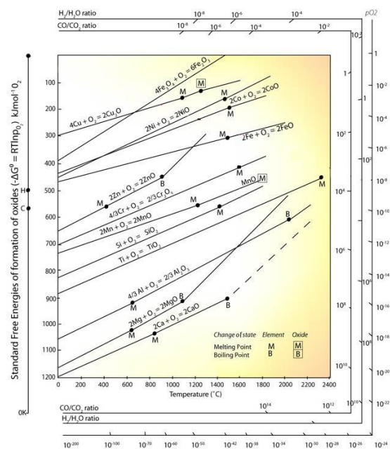
Fig. 4. Ellingham diagram [16]
