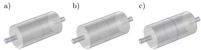
Fig. 10. Installation categories of the muffler: a) class a, b) class b, c) class c.
