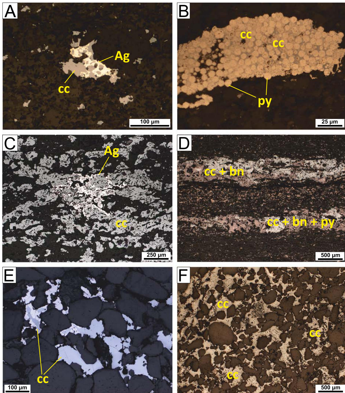
Text-fig. 2. Different types of copper ores from the Nowa Sol deposit. A – Nowa Sól C15 borehole, carbonate ore, native silver intergrowths (Ag) in a chalcocite aggregate (cc); B – Nowa Sól C25 borehole, carbonate ore, framboidal pyrite (py) cemented with chalcocite (cc); C – Nowa Sól C30 borehole, shale ore, massive chalcocite mineralization (cc) with native silver intergrowths (Ag); D – Nowa Sól C30 borehole, shale ore, chalcocite-bornite (cc + bn) and chalcocite-bornite-pyrite (cc + bn + py) veinlets following the Kupferschiefer lamination; E – Nowa Sól C30 borehole, sandstone ore, chalcocite (cc) filling intergrain spaces in the Weissliegend; F – Nowa Sól C30 borehole, sandstone ore, massive chalcocite mineralization (chalcocite cement; cc) in the top part of the Weissliegend.
