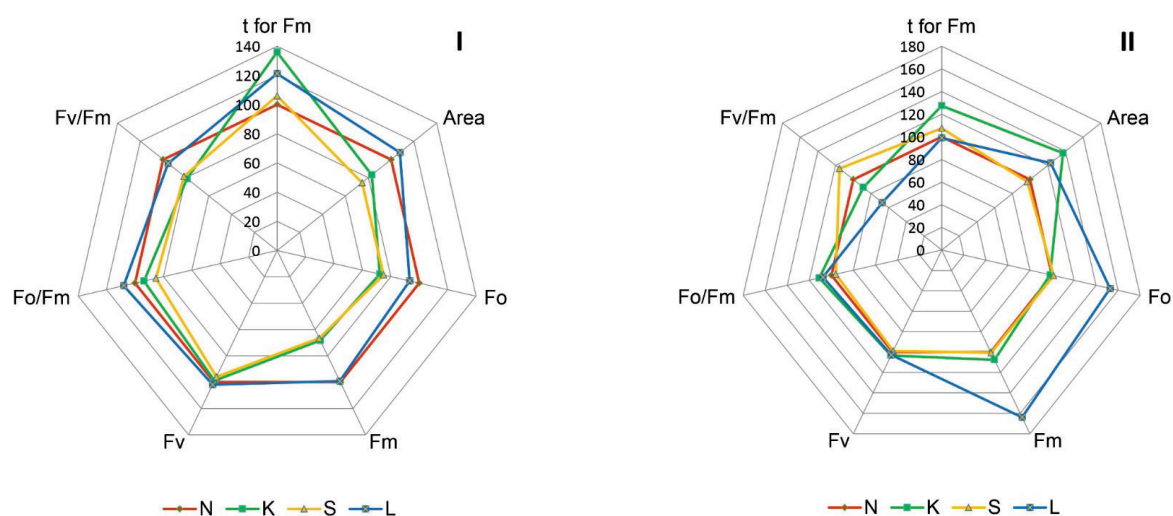
Fig. 1. Radar charts showing changes in the values of seven selected parameters of chlorophyll fluorescence in July (I) and in August (II); N, K, S, L as in Photo 1; source: own study
