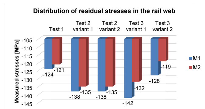
Fig. 14. Distribution of average residual stresses in the rail web in individual tests
