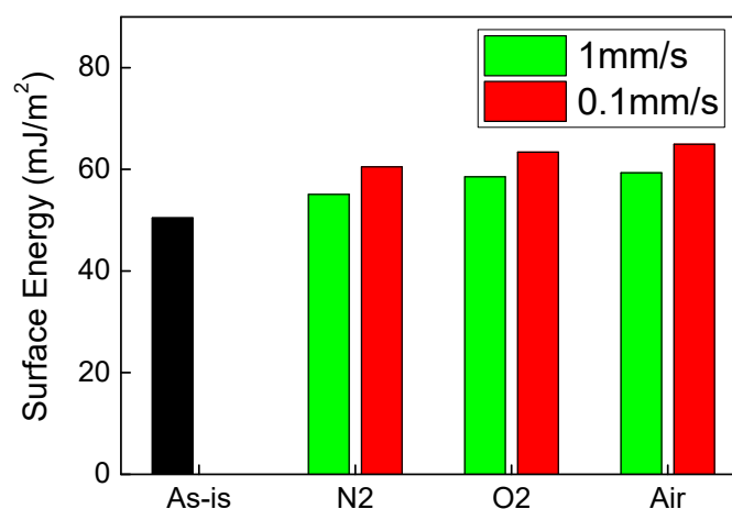
Fig. 4. Surface free energy of the Zn-Mg-Al coatings before and after the AP plasma treatment with different process gases and irradiation times
