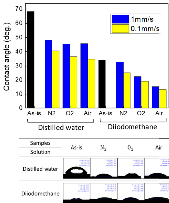
Fig. 3. Contact angles of the Zn-Mg-Al coatings before and after the AP plasma treatment with different process gases and irradiation times
