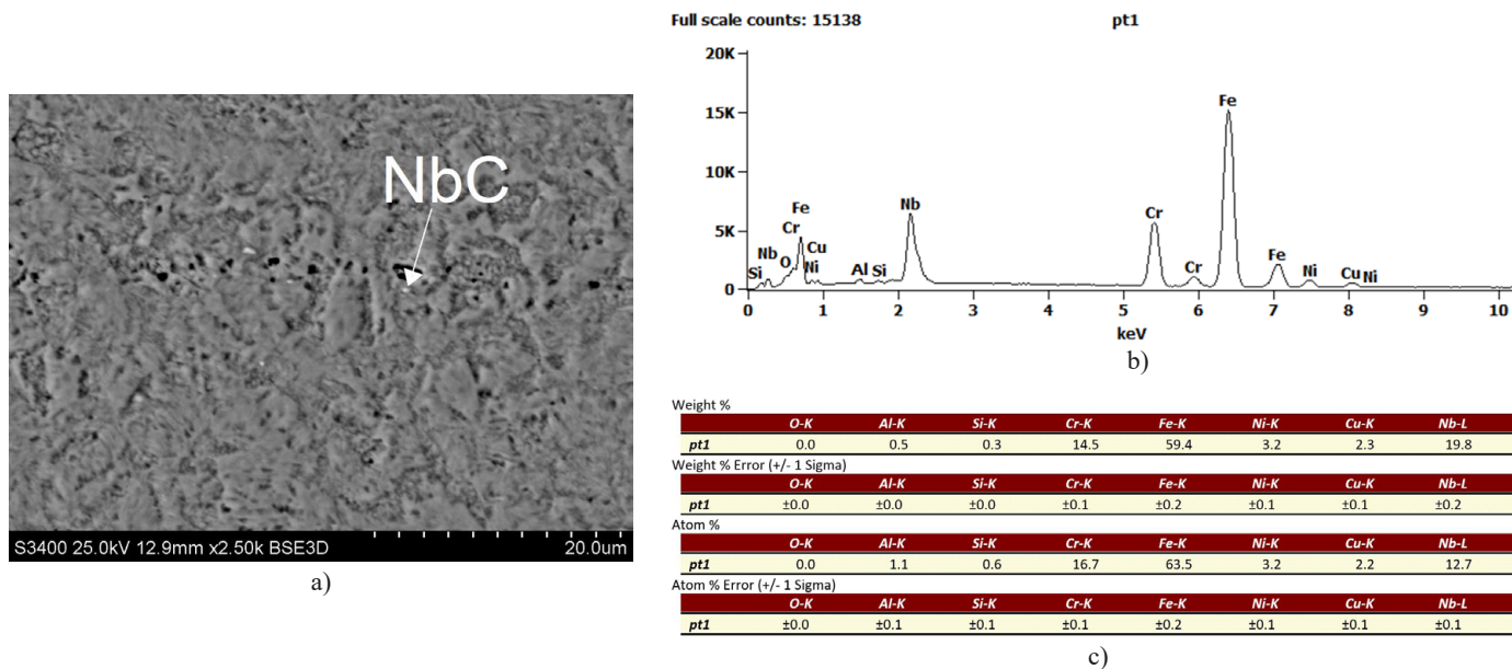
Fig. 9. SEM image of the heat affected HAZ2
