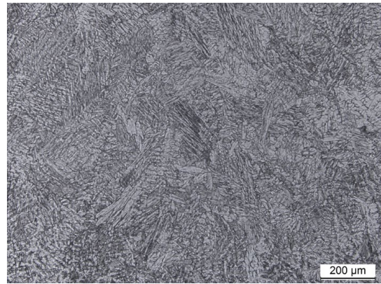
Fig. 5. Fusion weld microstructure of the welded joint 2 – martensite matrix with \delta -ferrite at grain boundaries
