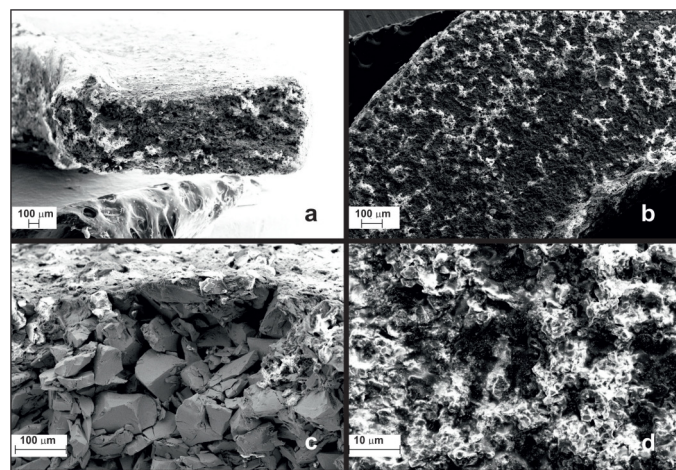
Fig. 7. image for composite covered high temperature varnish: a) general view, b) composite surface, c) composite cross-section, d) enlargement of the composite surface
