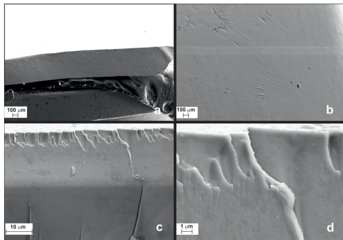
Fig. 4. SEM image for \text{Fe}_{70}\text{B}_{20}\text{Y}_5\text{Nb}_4\text{Mo}_1 alloy: a) general view, b) plate surface, c) plate cross-section, d) enlargement of the plate cross-section
