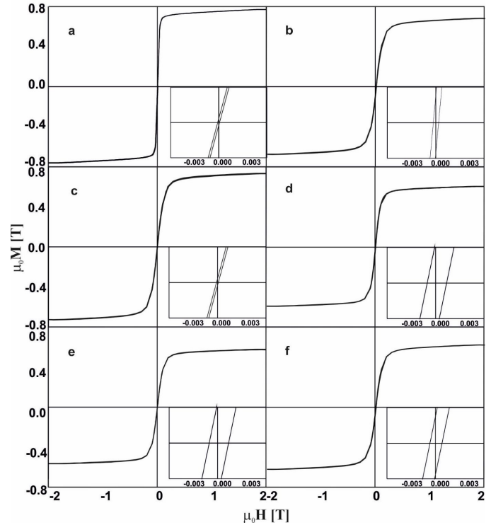
Fig. 14. Static magnetic hysteresis loops for: a) alloy after solidification, b) amorphous powder 50–100 μm, c) amorphous powder 50–100 μm after annealing 793 K/30 min, d) composite with 0.5% resin (annealing powder), e) composite covered high temperature varnish (annealing powder), f) composite covered high temperature varnish after HIP process
