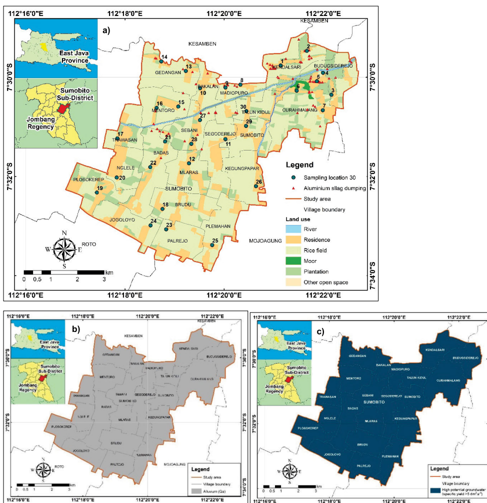
Fig. 1. Map of the study area in Sumobito District: a) dug wells' sampling site locations and land use, b) regional geology, c) potential of groundwater; source: own elaboration based on Santosa and Atmawinata (1992), and Nuzulliyantoro et al. (2020)
