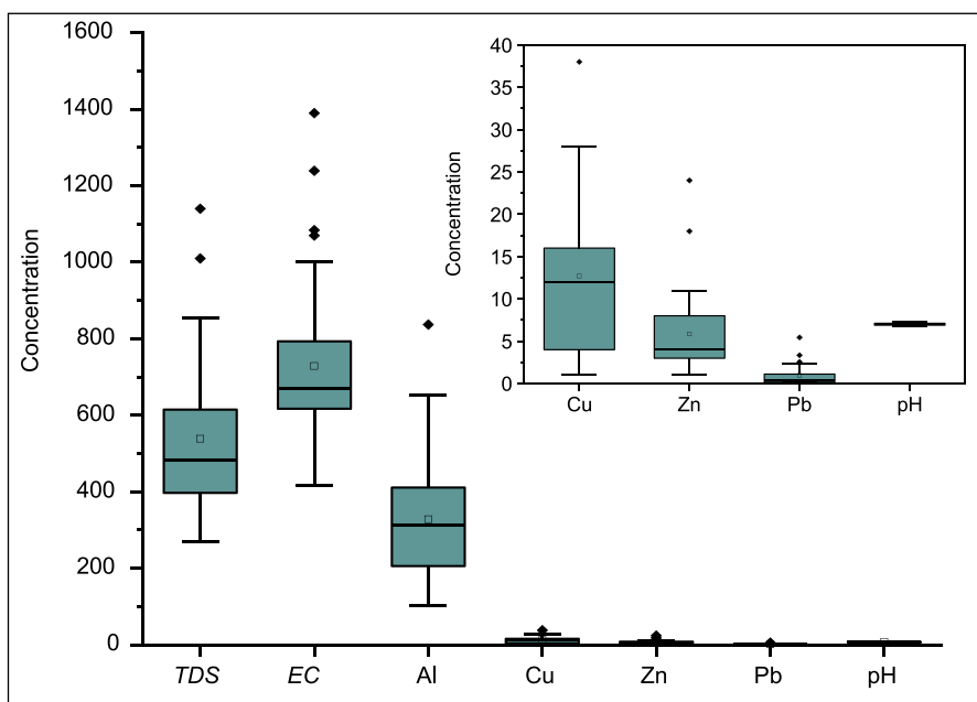
Fig. 3. Boxplot of shallow groundwater quality at Sumobito District; parameter units: TDS = mg·dm -3 ; EC = μS·cm -1 ; Al, Cu, Zn, Pb = μg·dm -3 ; source: own study
