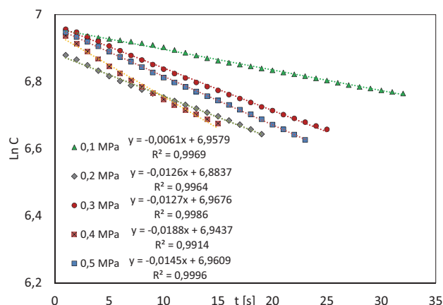
Fig. 11. Ammonia sorption curves in the kinetic range for a CW 50 nozzle for different supply pressures
