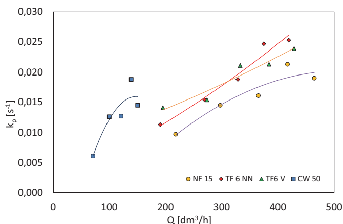
Fig. 13. Apparent sorption rate as a function of nozzle efficiency
