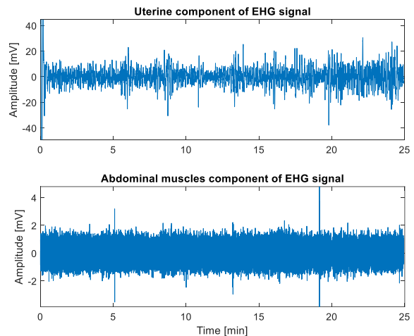
Fig. 4. Uterine and abdominal muscles components of the EHG signal registered during the 1 st stage of a labour
