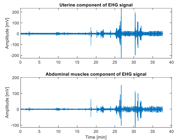
Fig. 3. Uterine and abdominal muscles components of the EHG signal registered during the 2 nd stage (active) of a labour in the woman trained in a childbirth school
