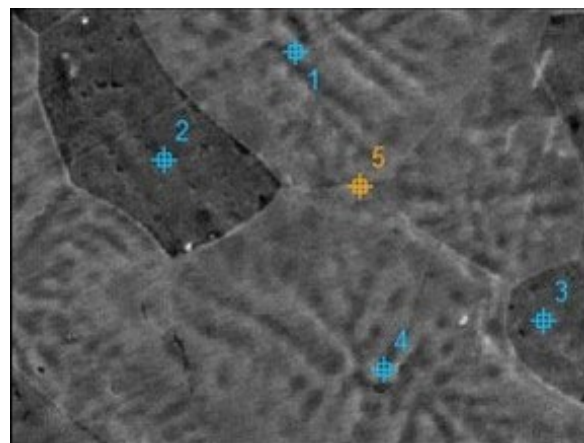
Fig. 4. SEM image of the FeNiCo 75 (AlSi) 25 alloy with chemical composition measurements points. The corresponding results are shown in TABLE 2
