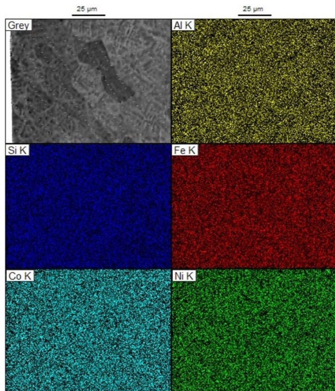
Fig. 3. The distribution of elements for FeNiCo 75 (AlSi) 25 alloy
