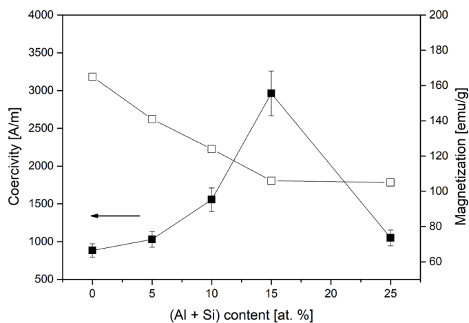
Fig. 5. The changes of coercivity and magnetization for (FeNiCo) 100-x (AlSi) x alloys as a function of (Al + Si) content
