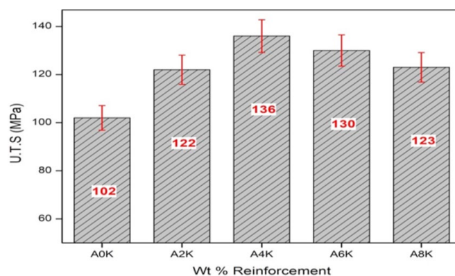
Fig. 7. Variation of U.T.S of MAS composite with wt% of kaolin particles
