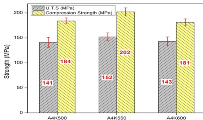
Fig. 8. Variation of Compression strength and U.T.S of the Al-Kaolin composite
