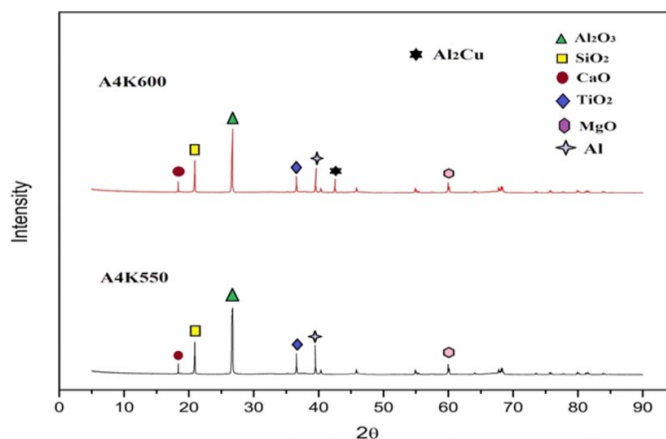
Fig. 4. XRD peaks for the single-mode cavity sintered Al-Kaolin composite at (a) 550°C and (b) 600°C
