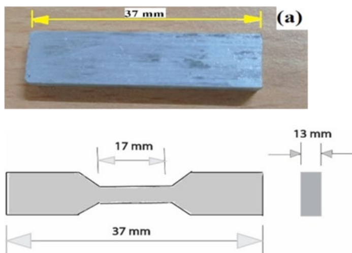
Fig. 2. Synthesized MAS composites for (a) Tensile test, (b) Hardness and Compression test
