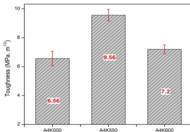
Fig. 10. Toughness of the single-mode cavity MAS sintered composite at different sintering temperatures
