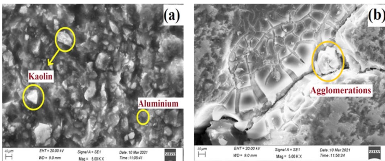
Fig. 5. SEM images for single-mode cavity MAS composite at (a) 550°C and (b) 600°C
