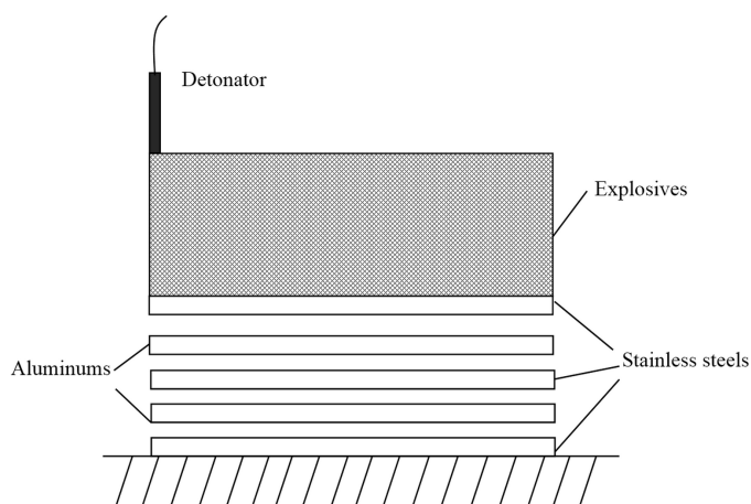
Fig. 1. Schematic diagram of explosive welding experimental device
