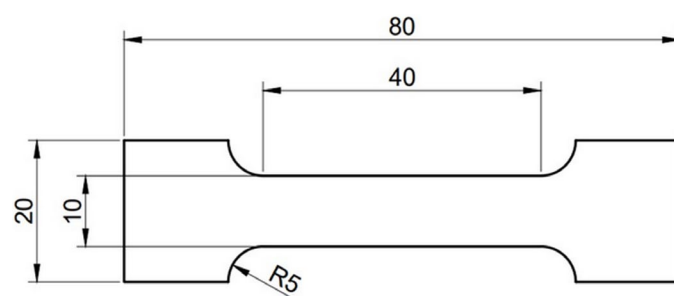
Fig. 2. Tensile sample size
