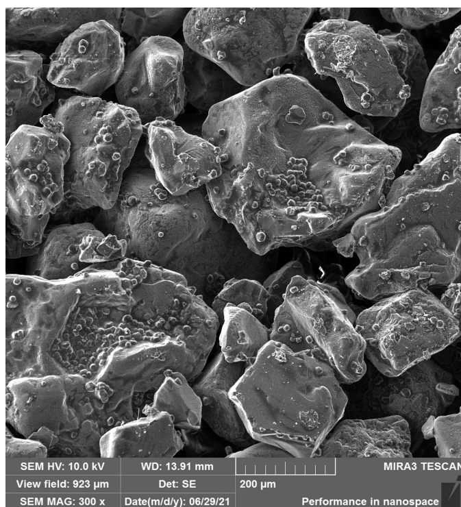
Fig. 14b. Sample of sand core mixture G after casting, magnification 300×
