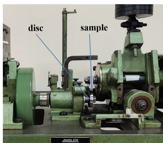
Fig. 5. Configuration of disc – sample contact
