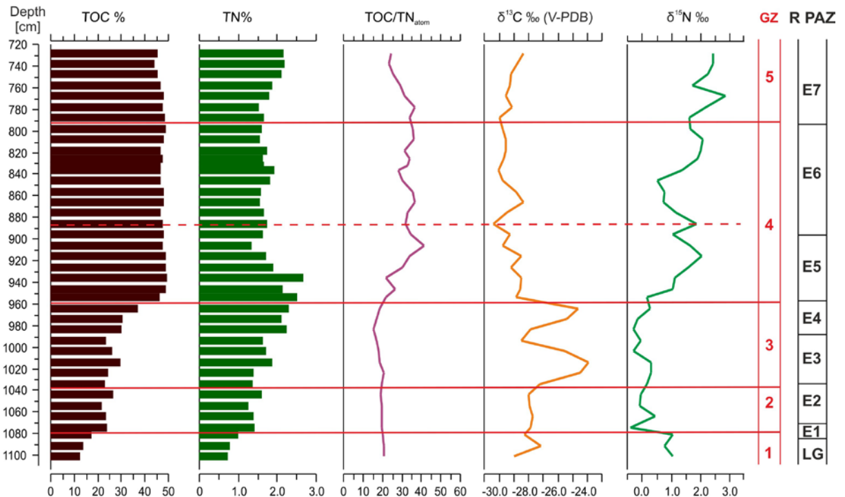
Text-fig. 8. Diagram of the results of isotopic analyses of sediments from the Ża-19 core against the division into RPAZs.
