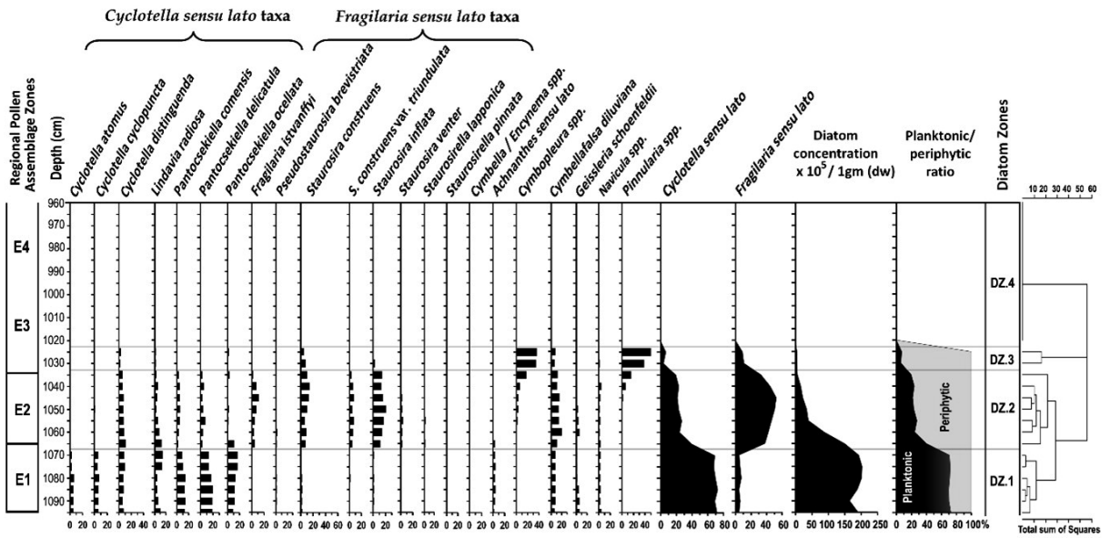
Text-fig. 7. Percentage diatom diagram of the Ża-19 profile with diatom valve concentration, planktonic and periphytic ratio and the diatom zones based on the cluster analysis.
