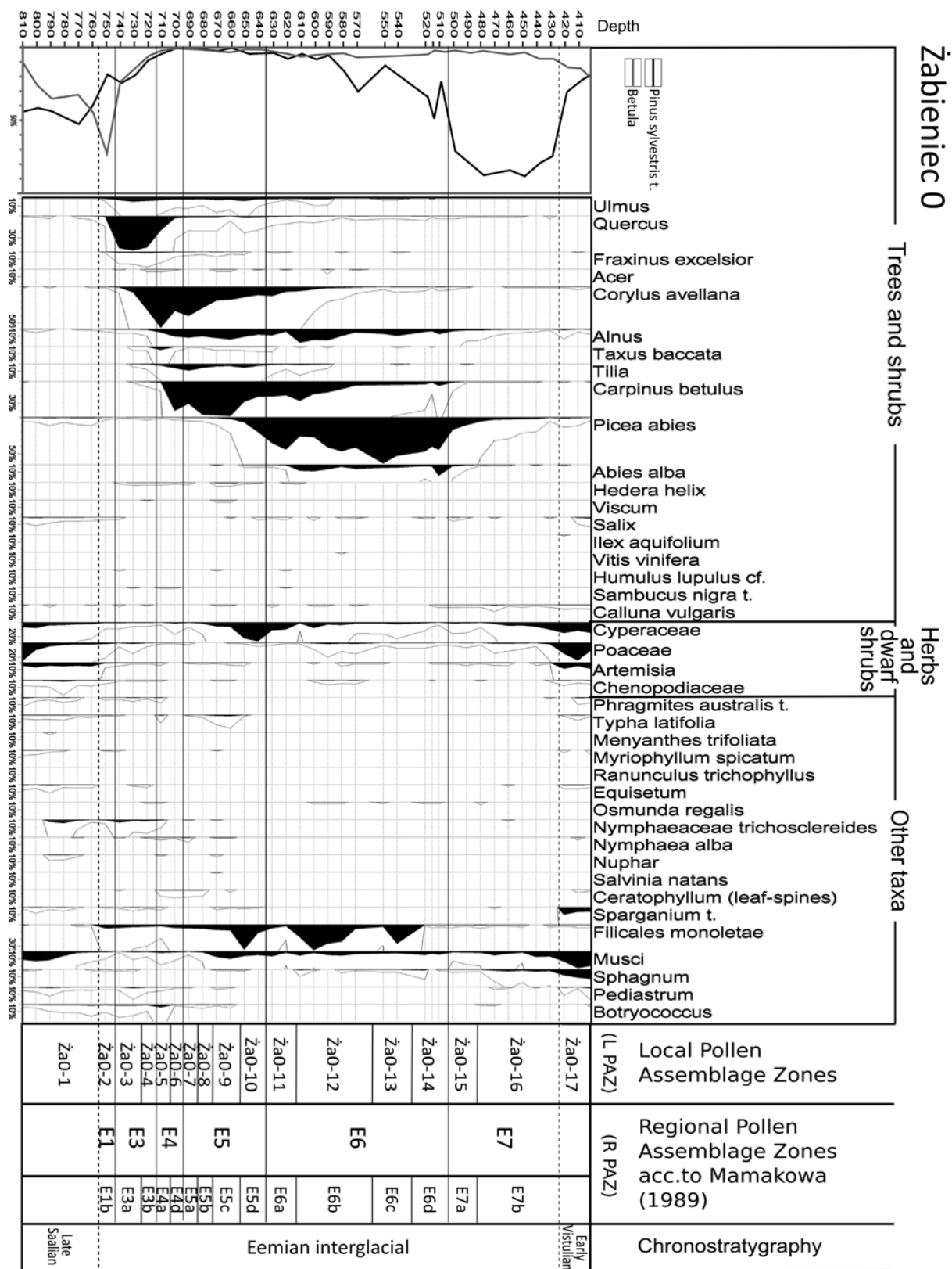
Text-fig. 3. Simplified percentage pollen diagram of the Ża-0 profile.
