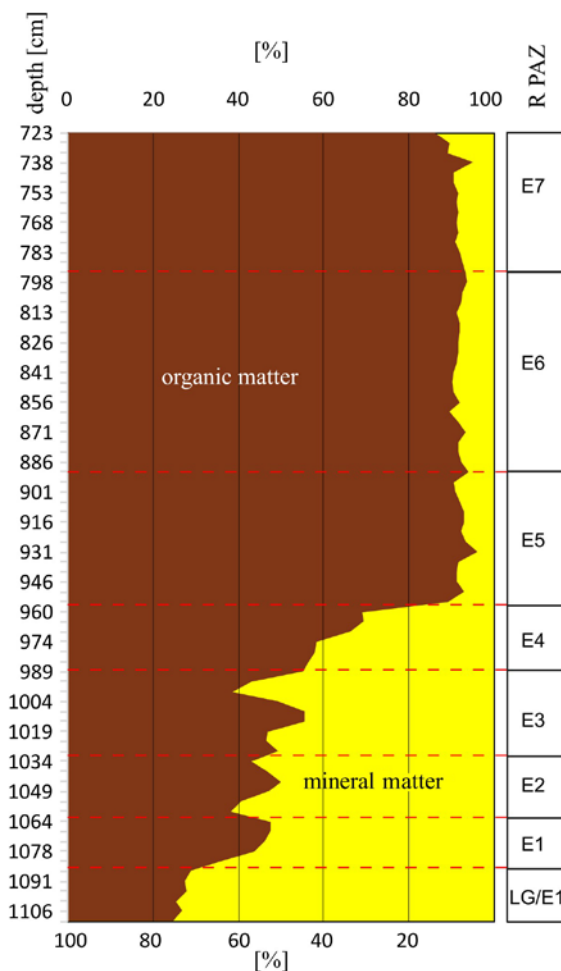
Text-fig. 9. Percentage share of mineral and organic matter in the Ża-19 core.
