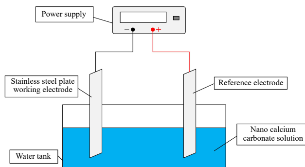
Fig. 6. Electrochemical fouling preparation system.
