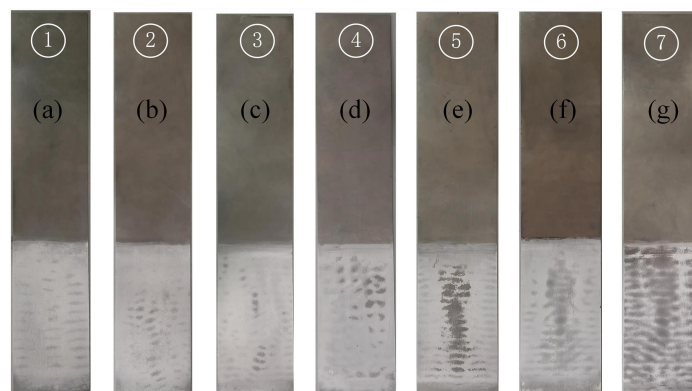
Fig. 10. Descaling results under different excitation modes: a)–c) single-frequency; d)–f) dual-frequency; g) triple-frequency.
