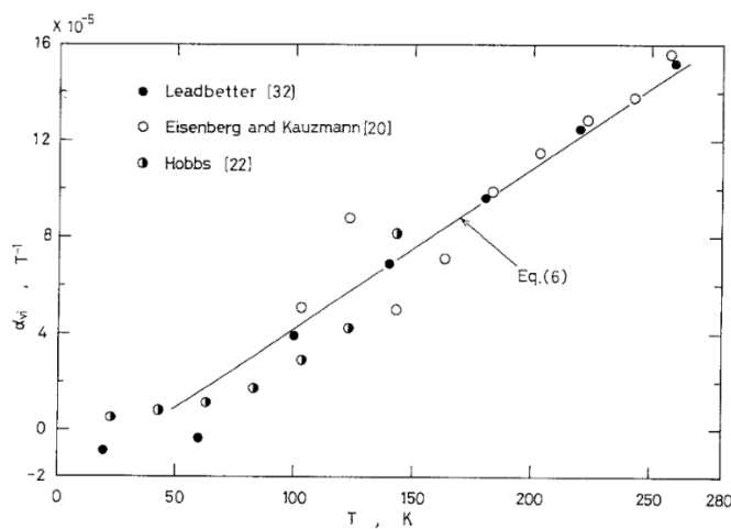
Figure 3: Cubic expansion coefficient as a function of temperature [21].
