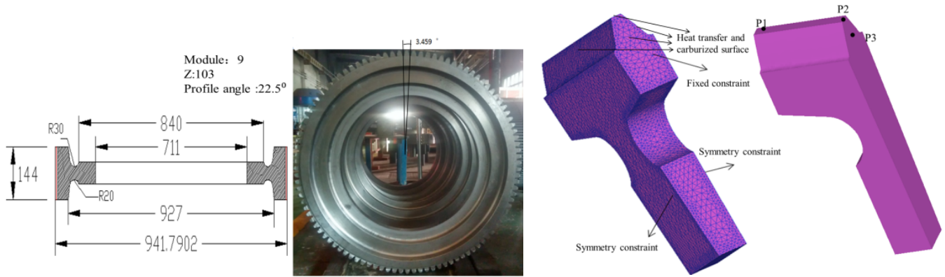
Fig. 1. Gear structure and analysis model
