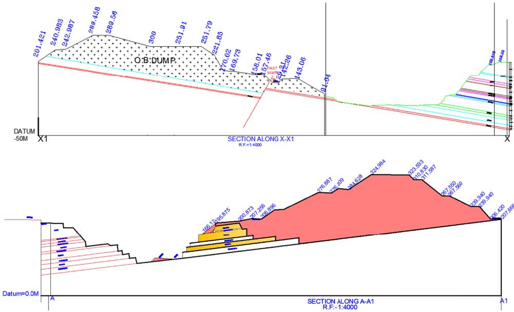
Fig. 18. Section of overburden dumps for Mine 2
