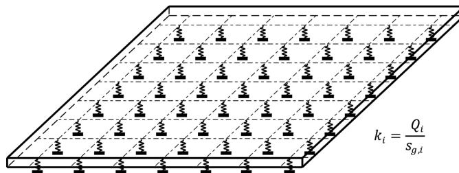
Fig. 4. Scheme of the consideration of the raft (slab) stiffness
