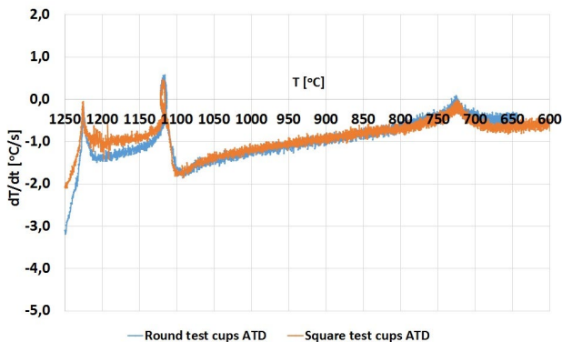
Fig. 17. Pathways of ATD curves of hypoeutectic cast iron in samplers of square and circular cross-sections
