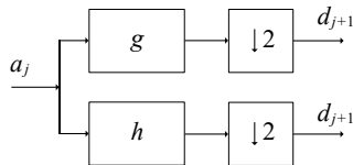
Fig. 7. Single level signal decomposition: h – low pass filter; g – high pass filter; ↓2 – decimation symbol.
