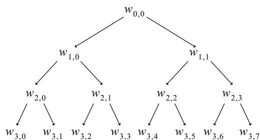
Fig. 10. Signal decomposition scheme using wavelet packets.
