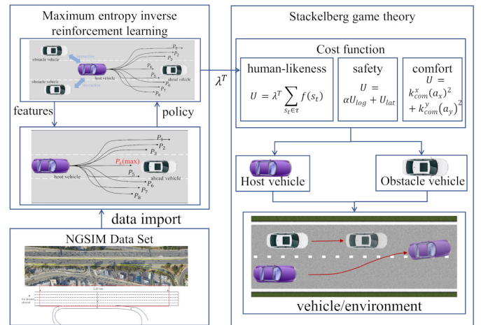
Fig. 2. Algorithmic framework for human-like driving decisions
