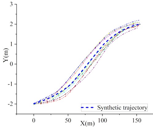
Fig. 9. Synthetic trajectory
