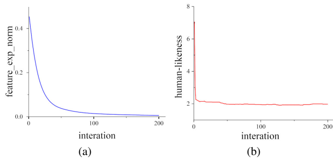
Fig. 7. Training process: (a) plot of trajectory feature expectation difference; (b) plot of human-likeness
