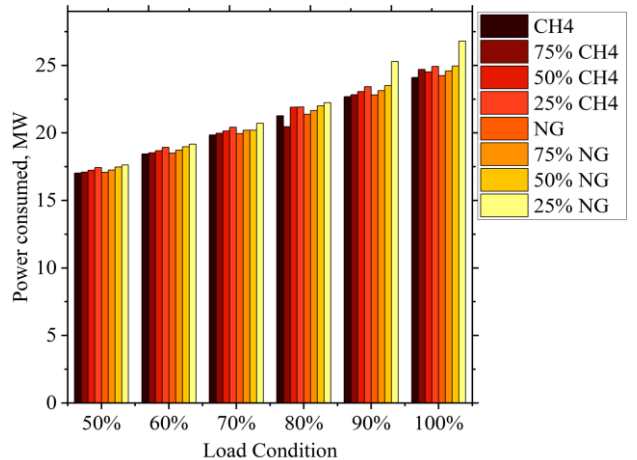
Fig. 9. Total power consumption of CCGT using different fuels and mixture of fuels with PCCS operated under different load conditions.
