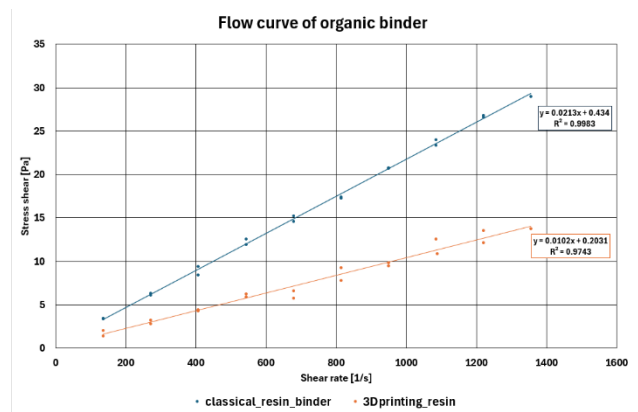
Fig. 1. Flow curves and dynamic viscosity values of the tested binders
