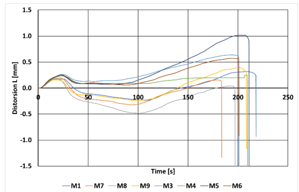
Fig. 8. Thermal deformation in the function of heating time
