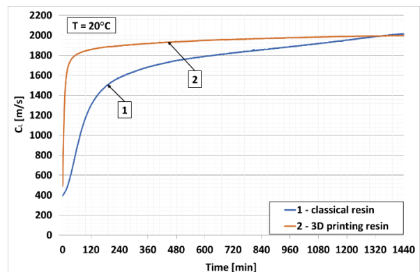
Fig. 2. Comparison of the course of changes in the velocity ( C_L ) of wave passage in the tested molding sands
