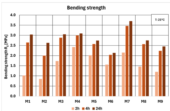
Fig. 4. Influence of hardening time on the bending strength of the tested molding sands
