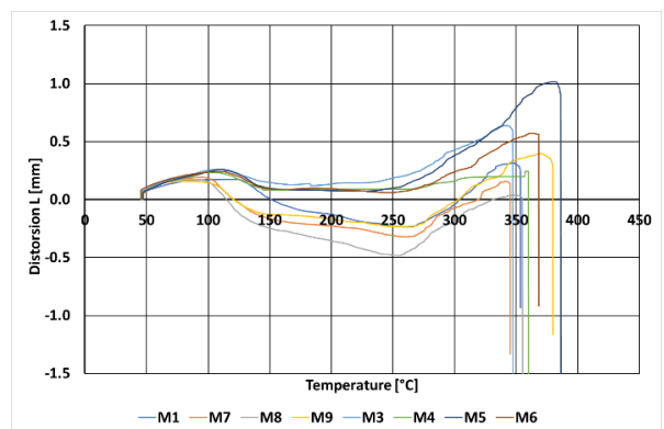
Fig. 9. Thermal deformation in the function of temperature
