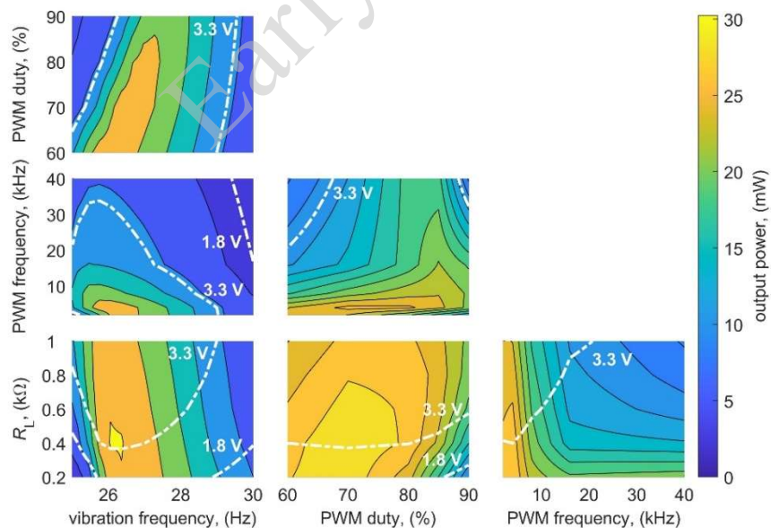
Fig. 10. Performance maps of the output power of electromagnetic energy harvester with bridgeless boost rectifier at 10 \text{ m/s}^2 . Each contour plot shows the dependency of output power on two variables of
