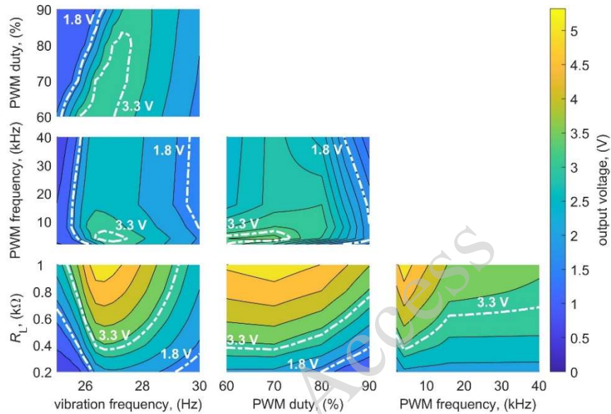
Fig. 11. Performance maps of the output voltage of electromagnetic energy harvester with bridgeless boost rectifier at 10 m/s^2 . Each contour plot shows the dependency of output voltage on two variables of the four, with the remaining two variables equal as in Table 3 (vibration frequency – 26.7 Hz, PWM duty – 70%, PWM frequency – 4 kHz, R_L – 400 \Omega )
