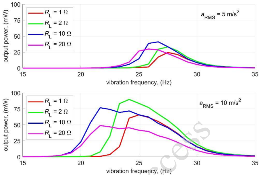
Fig. 4. Measured output power at different loads during a frequency sweep from 35 to 15 Hz, with excitation accelerations of 5 and 10 m/s 2
