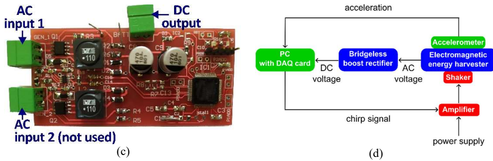
Fig. 2. Bridgeless boost rectifier for energy harvesting (a); zero-crossing detection circuit and control circuit for proposed boost converter (b); manufactured prototype (c); laboratory setup (d)
