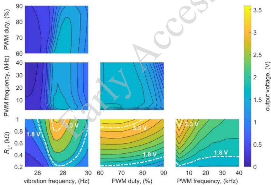
Fig. 7. Performance maps of the output voltage of electromagnetic energy harvester with bridgeless boost rectifier at 5 m/s 2 . Each contour plot shows the dependency of output voltage on two variables of the four, with the remaining two variables equal as in Table 3 (vibration frequency – 27.9 Hz, PWM duty – 60%, PWM frequency – 4 kHz, R_L – 200 \Omega )
