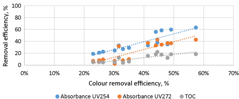
Fig. 3. Correlations between colour removal efficiency and absorbance in UV 254 , UV 272 or total organic carbon in coagulation by PAX XL3
