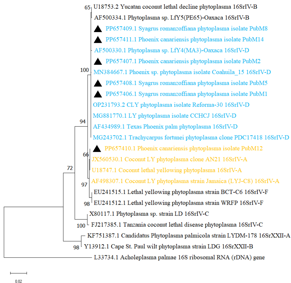
Fig. 4. Phylogeny of phytoplasma 16S rRNA gene sequences inferred by Maximum Likelihood. For the analysis, 24 representative sequences deposited in GenBank® and a total of 1248 base pairs were used. The sequences of phytoplasma isolates from Puebla are denoted with ▲. The trust level of the internal nodes is displayed next to the branches
