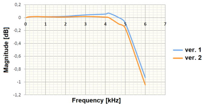
Fig. 8. Pass-band filter frequency response for TLV2462 and OP275 operational amplifiers in two versions of selection of passive components
