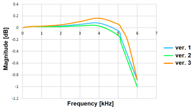
Fig. 7. Pass-band filter frequency response for TL072 operational amplifiers in 3 versions of selection of passive components
