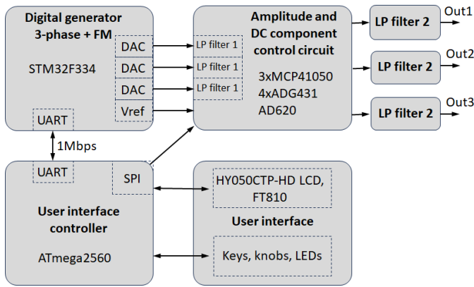
Fig. 1. Block diagram of the digital signal controller for an experimental magnetotherapy device
