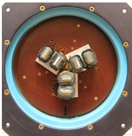
Fig. 12. View of the interior of a handmade magnetotherapy applicator (visible star configuration of coils)
