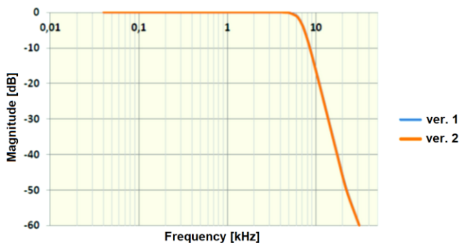
Fig. 9. Full-range filter frequency response for TLV2462 and OP275 operational amplifiers in two versions of selection of passive components (both curves are almost identical and overlap)
