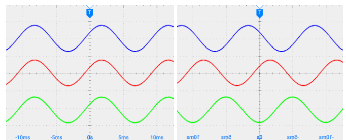
Fig. 10. Oscillograms of the 3-phase output signal for: a) stationary magnetic field, b) counter-clockwise turning magnetic field
