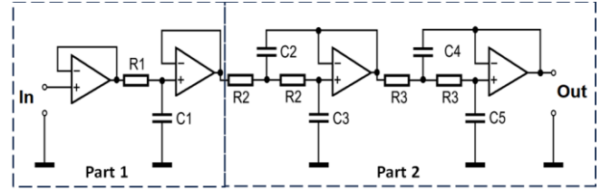
Fig. 4. The diagram of the 5th order reconstruction filter for one channel, divided into two parts 1 and 2
