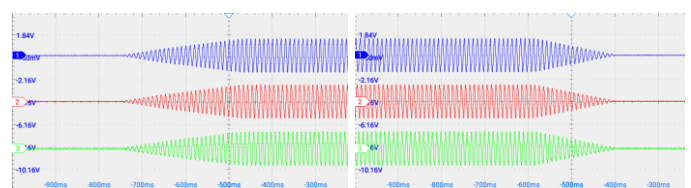
Fig. 11. 3-phase signals without DC component during soft start (left) and soft-stop (right)
