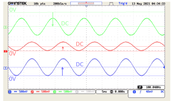
Fig. 3. Three example signals: a) large negative DC component, output signal only negative, b), c) positive DC component equal to the signal amplitude
