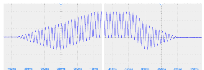
Fig. 11. Signal of one phase with a positive DC component added during soft start (left) and soft-stop (right)
