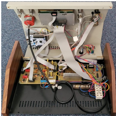
Fig. 7. Internal view of the realized controller
