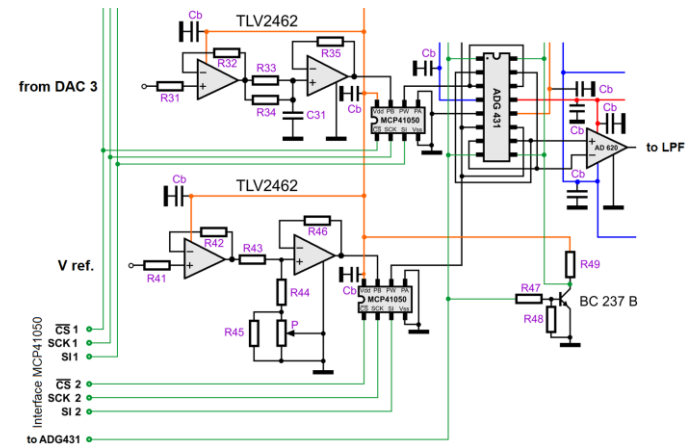
Fig. 2. A part of the diagram of the amplitude and DC component control circuit for channel number 3
