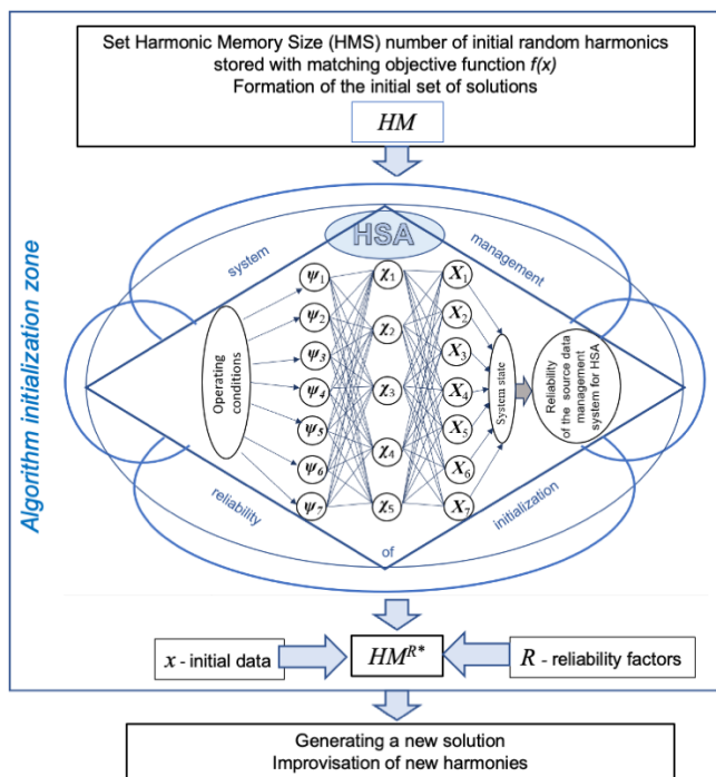
Fig. 2. Detailed visualization of the systematic modification of the harmony search algorithm (HSA) (source own)
