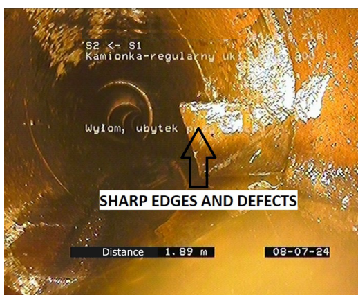
Fig. 3. Example of sharp edges and defects
