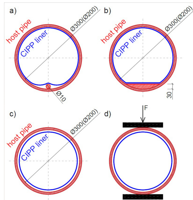
Fig. 4. Schematic diagrams of laboratory models: a) model with a fold, b) model with deposits, c) reference model, d) research scheme
