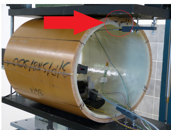
Fig. 11. Testing of a sample with a fold
