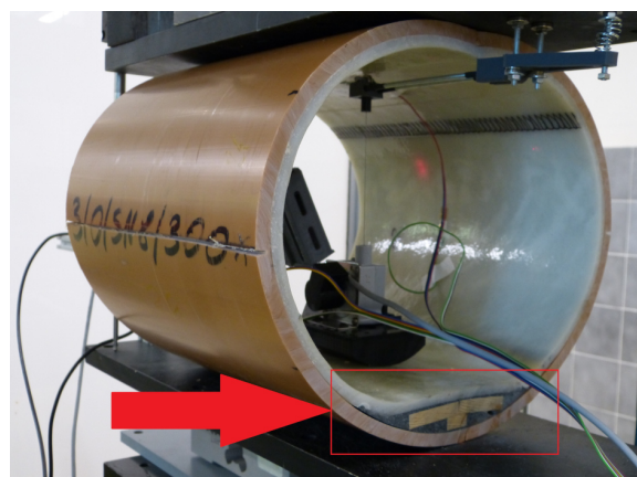
Fig. 9. Testing of a sample with sediments
