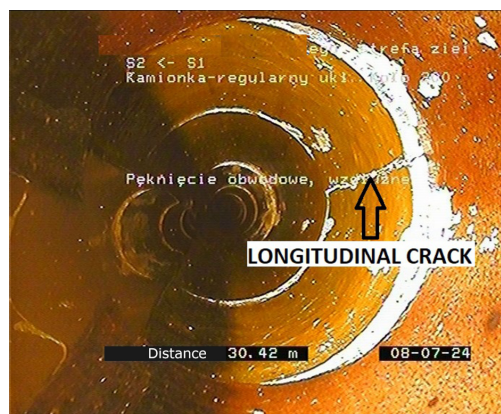
Fig. 1. Example of a longitudinal crack
