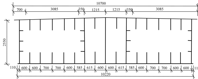
Fig. 3. Cross-sectional diagram of the main bridge of Jinzhou Bridge (2) (mm)
