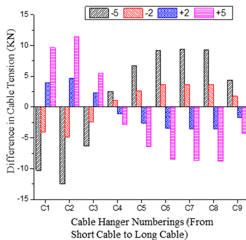
Fig. 13. The change in cable stiffness results in variations in the cable tension
