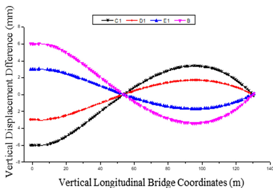
Fig. 24. Effects of overall temperature difference on vertical displacement of the main beam nodes
