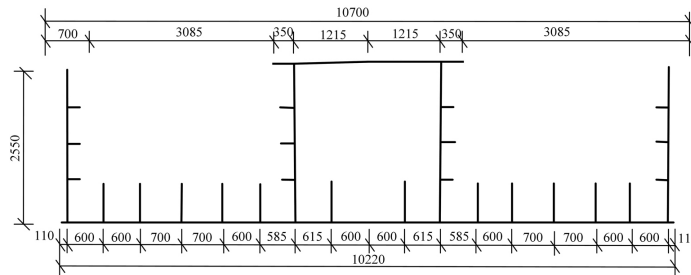
Fig. 4. Cross-sectional diagram of the main bridge of Jinzhou Bridge (3) (mm)
